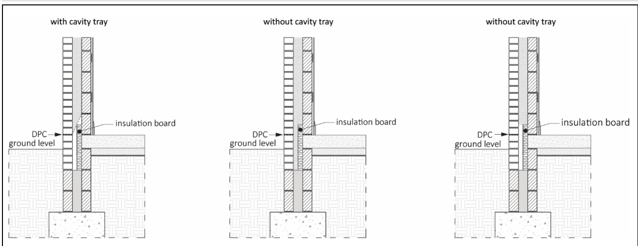
Figure 3 Existing insulation at ground floor slab and external wall junction
