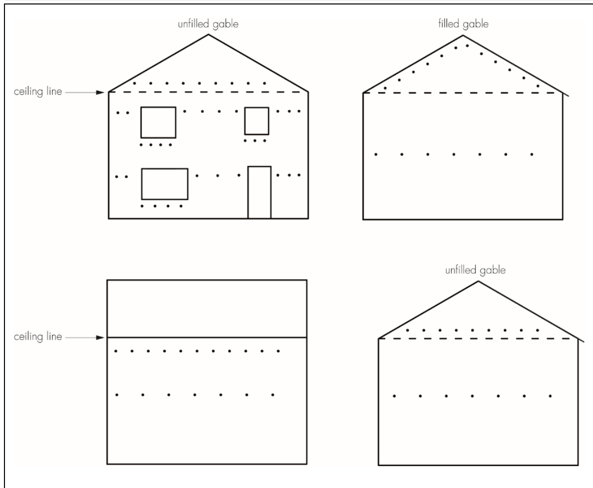
Figure 1 Standard drilling pattern
